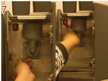
7 Reassemble the mixer unit into the powder module. Turn the knob to the left to lock. Reconnect tube to the mixer. Push power button to turn on the powder module.
